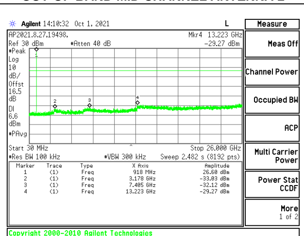
OUT-OF-BAND HIGH CHANNEL ANTENNA 2
