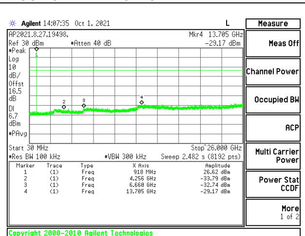
OUT-OF-BAND MID CHANNEL ANTENNA 2
