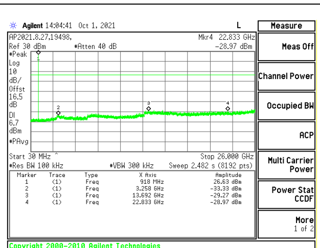
OUT-OF-BAND LOW CHANNEL ANTENNA 2
