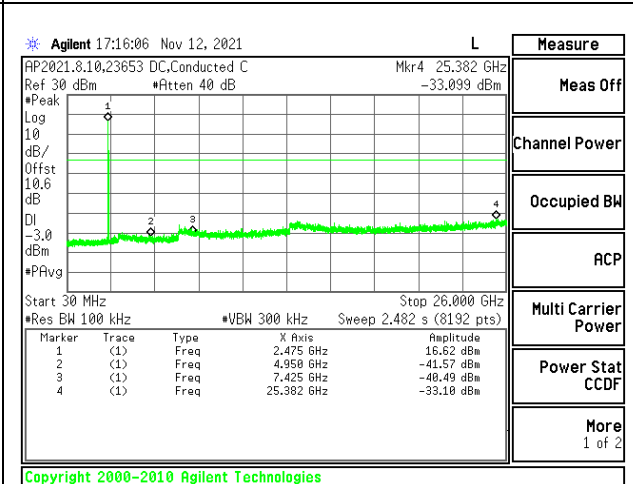
OUT-OF-BAND 2475MHz ANTENNA 1
