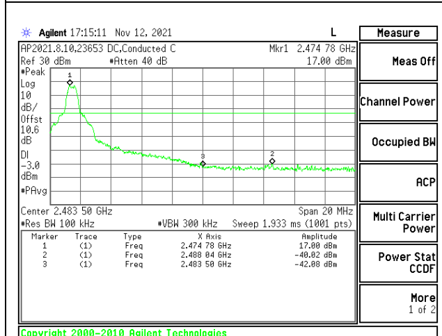
2475MHz BANDEDGE ANTENNA 1
