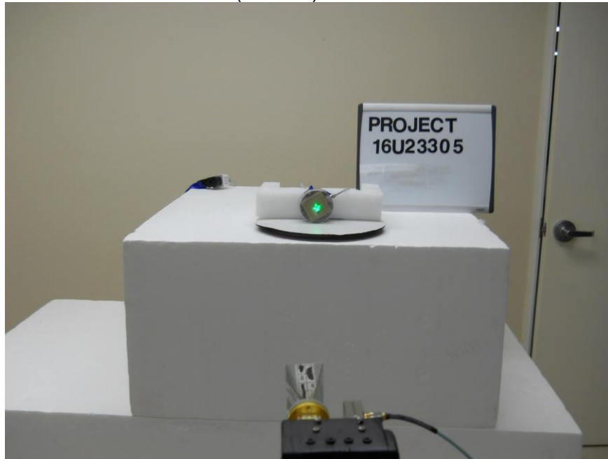
RADIATED EMISSIONS (FRONT)
