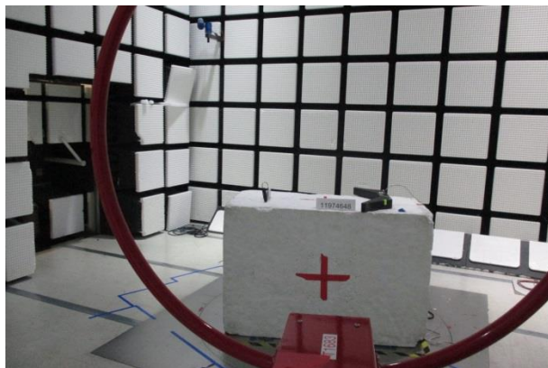
RADIATED FRONT PHOTO (BELOW 30MHz)
