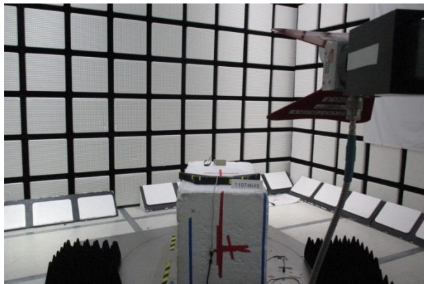
RADIATED FRONT PHOTO (ABOVE 1-18 GHz)
