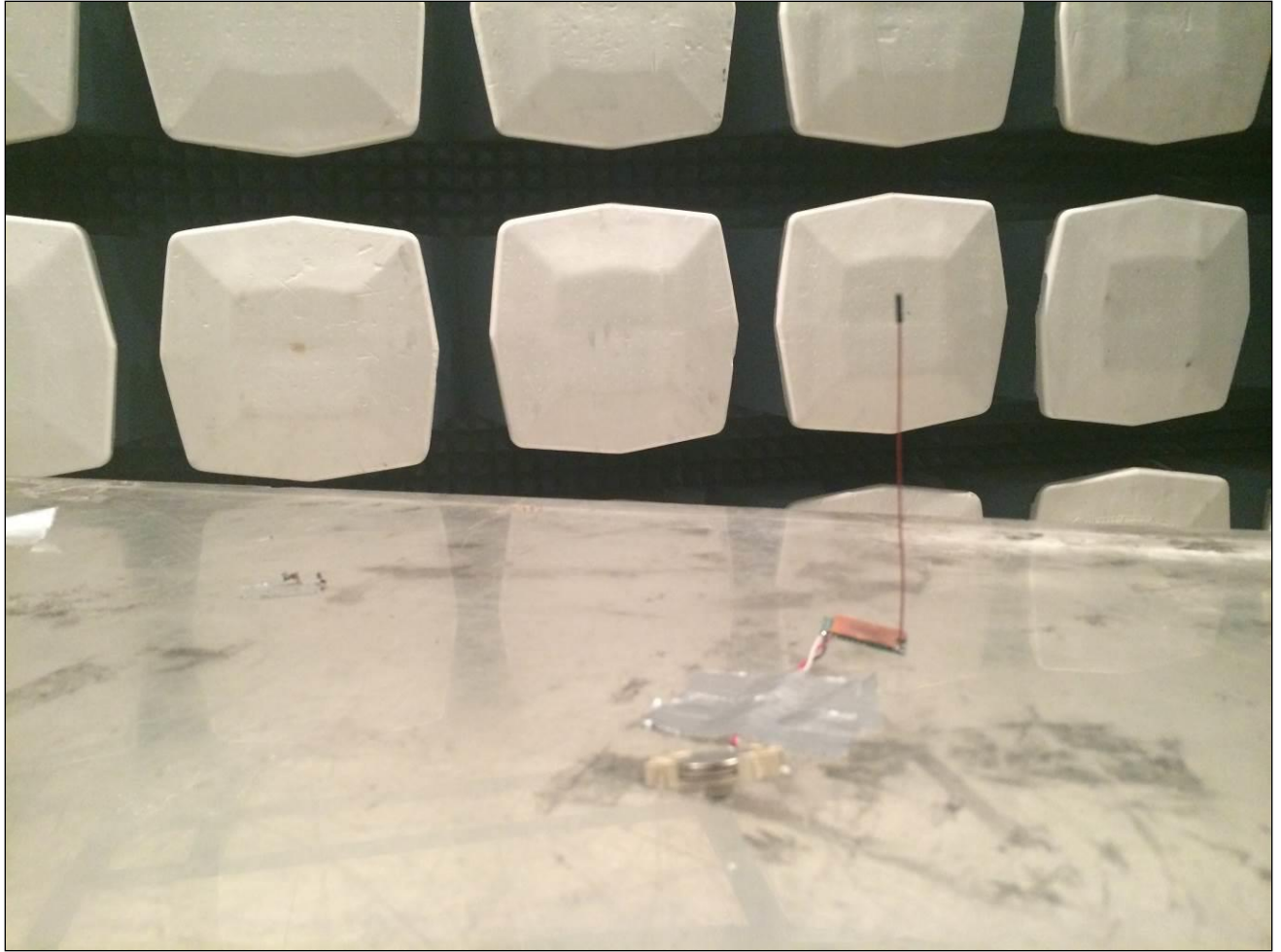
Photograph 1. Field Strength of Fundamental and Harmonics, Test Setup
