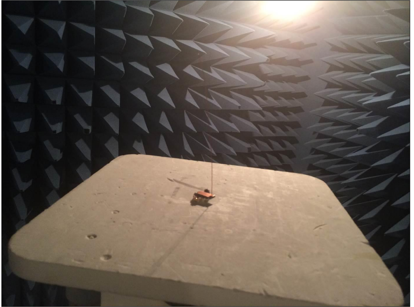
Photograph 2. Spurious Emissions, Above 1 GHz, Test Setup
