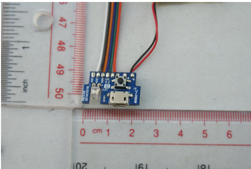
EUT MAIN BOARD TOP VIEW 5
