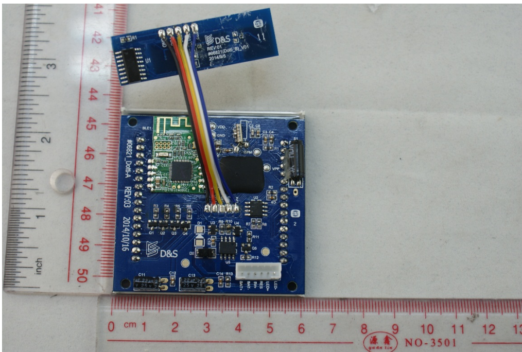
OPEN THE EUT PHOTO 2
