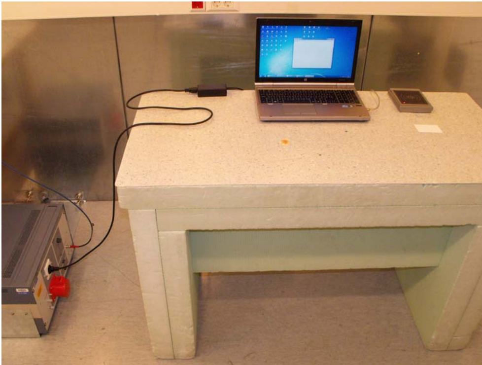
Figure 1: Conducted emission test – 150 kHz to 30MHz
