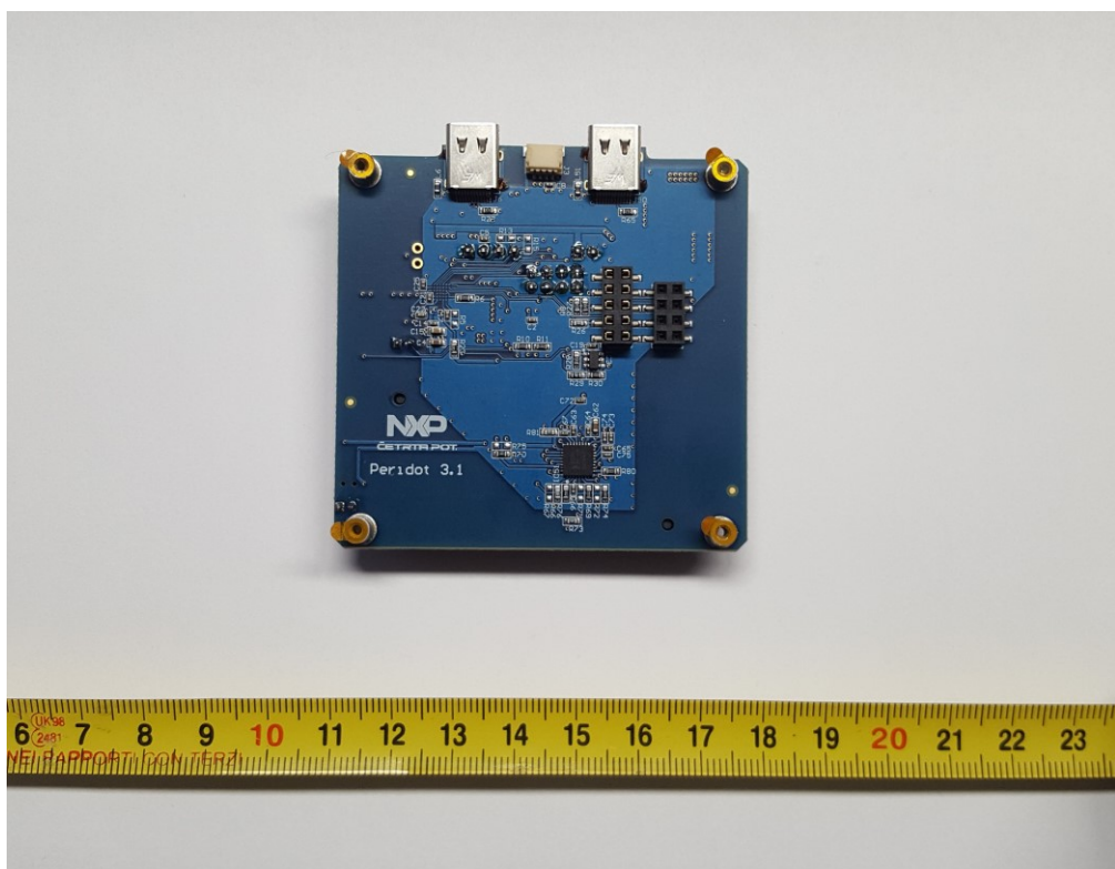
Figure 2: CLRD730 reader internal - bottom side
