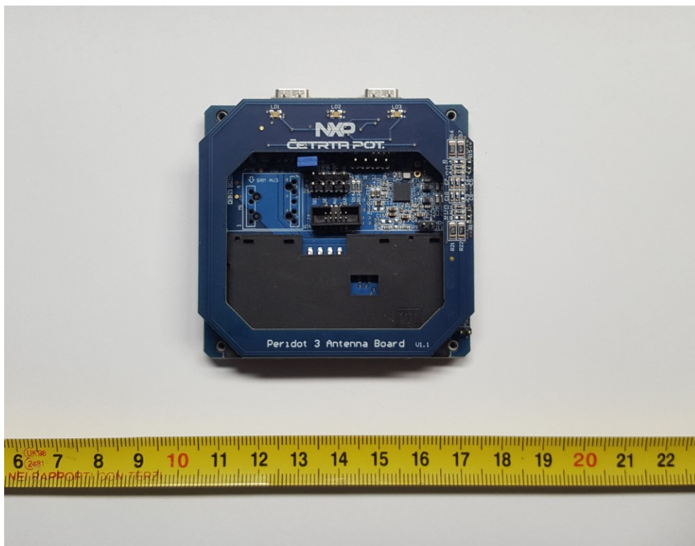
Figure 1: CLRD730 reader internal - top side
