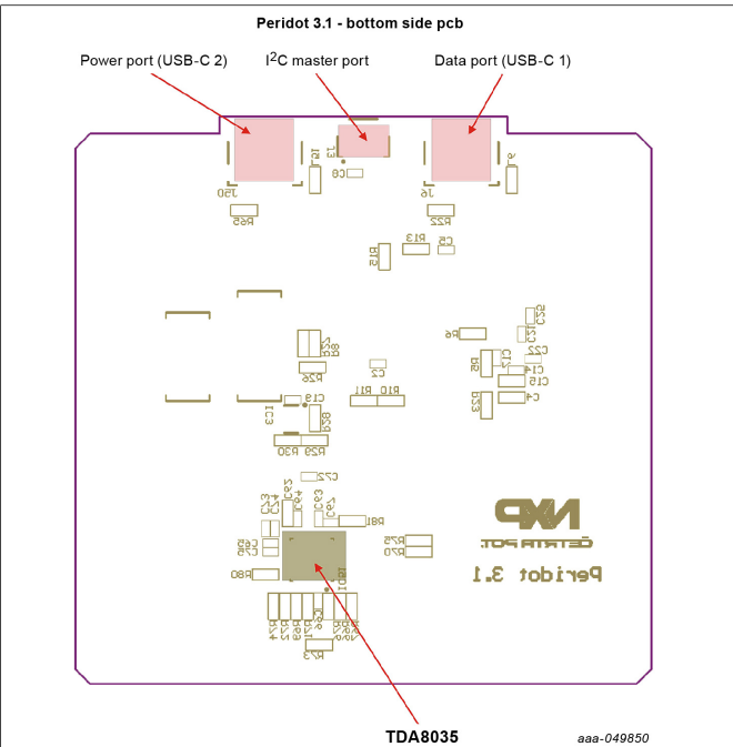
Figure 7. PCB main board - bottom side
