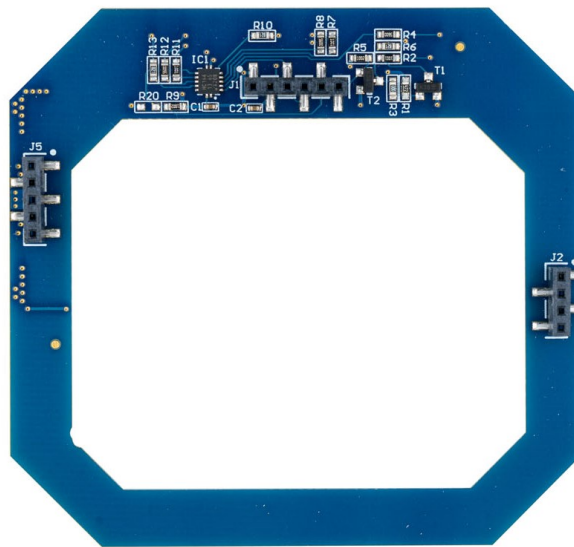
Figure 10. Antenna bottom
