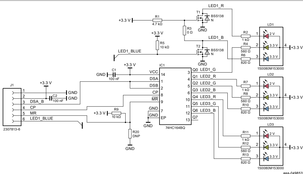
Figure 11. Header J1 for connecting LEDs to main board Peridot 3.1
