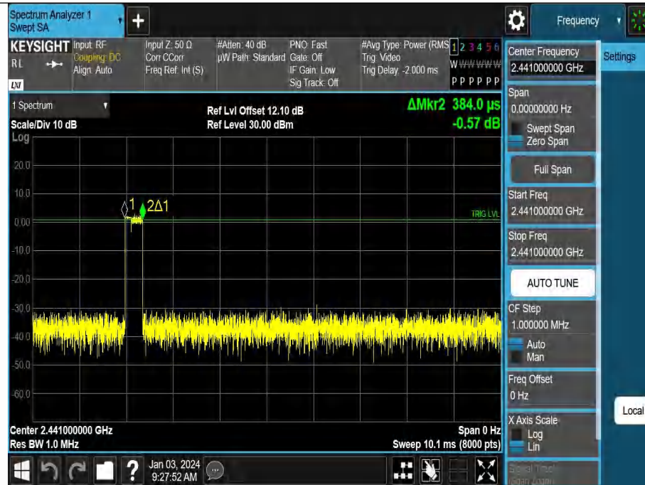
3DH1-Ant1-Hop-PASS
