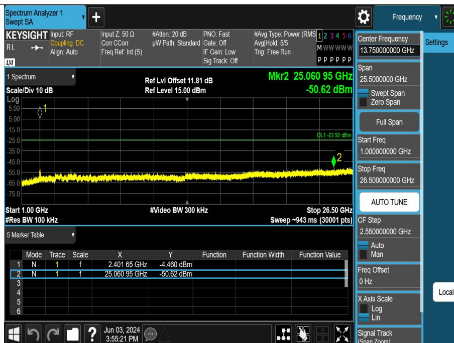
DH5-Ant1-2402-1000~26500-PASS
