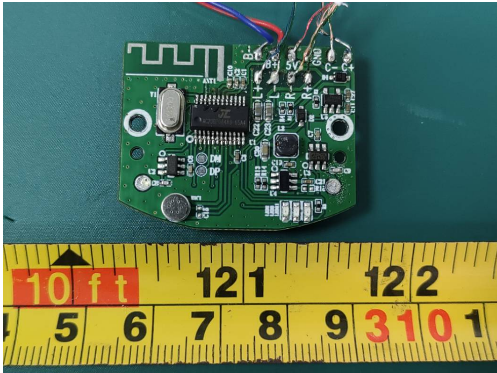
Bluetooth Antenna
