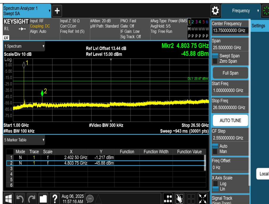
DH5-Ant1-2402-1000~26500-PASS
