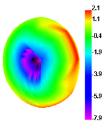
Bluetooth 78 TRP
