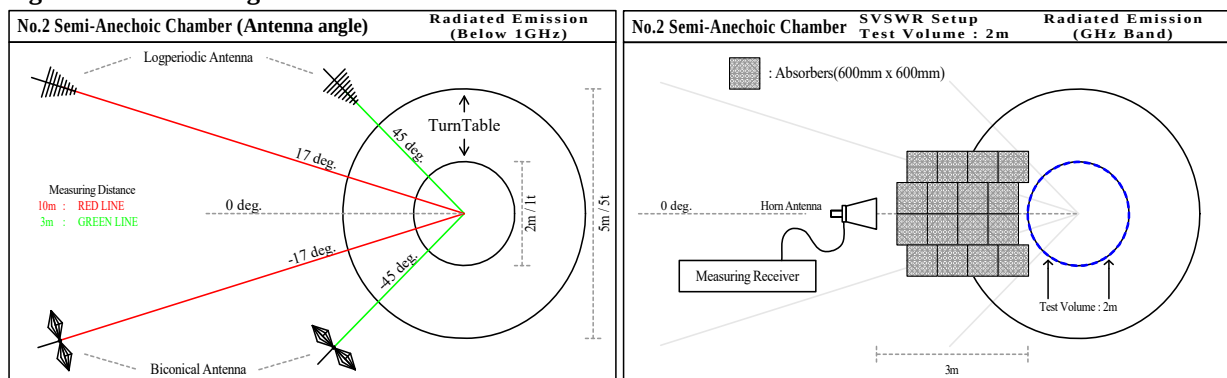
Figure 2. Antenna angle
