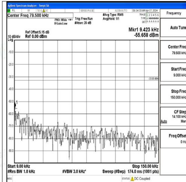
Band12_1.4MHz_QPSK_23017_1RB#0_0.009~0.15_0.09~0.15
