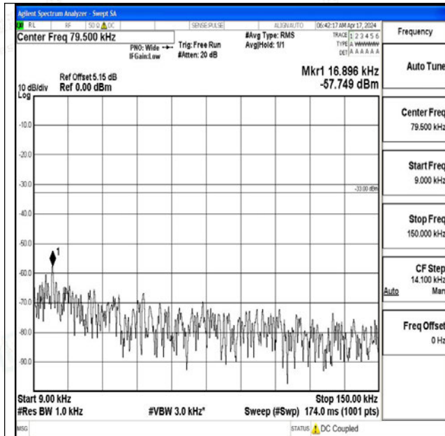
Band12_3MHz_QPSK_23095_1RB#0_0.009~0.15_0.009 ~0.15
