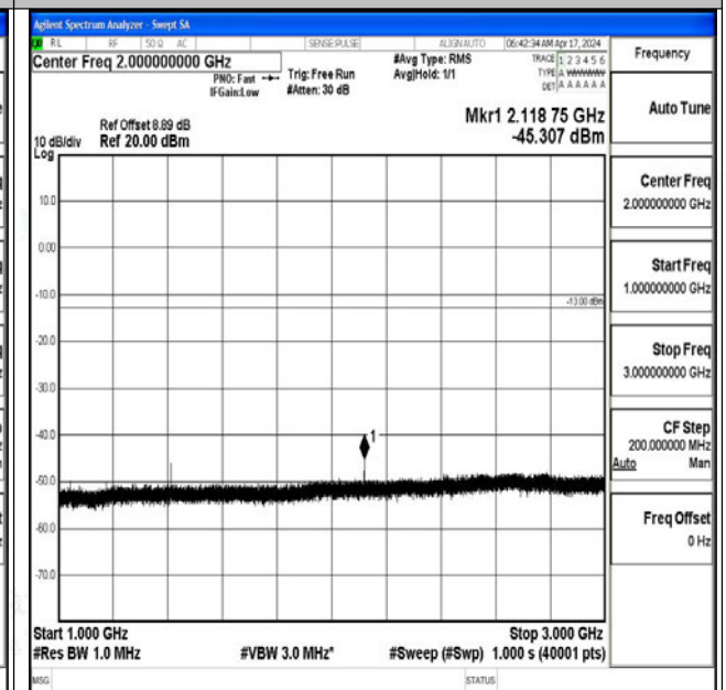
Band12_3MHz_QPSK_23095_1RB#0_1000~3000_1000 ~3000
