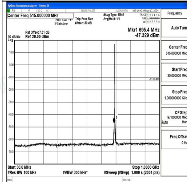
Band12_1.4MHz_QPSK_23017_1RB#0_30~1000_30~1000
