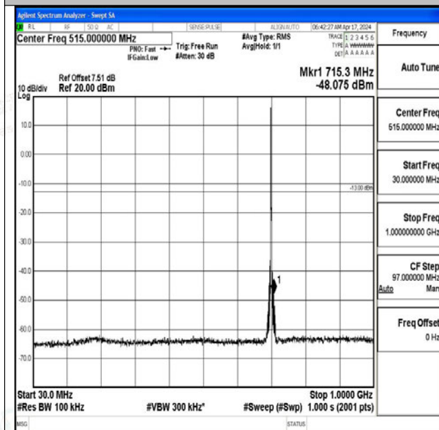
Band12_3MHz_QPSK_23095_1RB#0_30~1000_30~100 0
