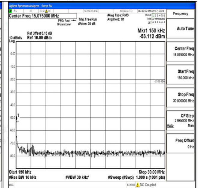
Band12_3MHz_QPSK_23095_1RB#0_0.15~30_0.15~30
