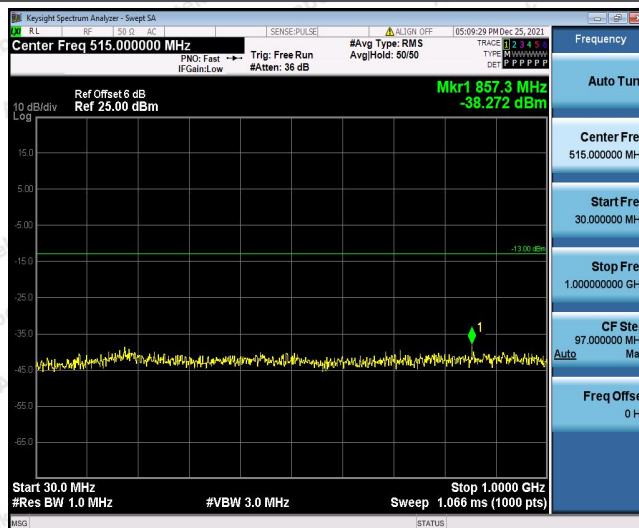
Band66-15MHz-QPSK-132322-1RB#0-Range2:1000~10000MHz
