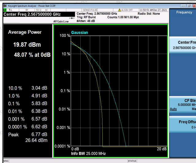
Band41-5MHz-QPSK-40365-25RB#0
