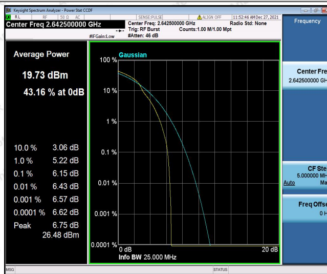
Band41-5MHz-16QAM-41115-25RB#0
