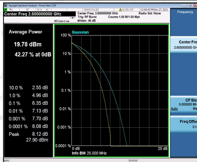
Band41-10MHz-QPSK-41115-1RB#0
