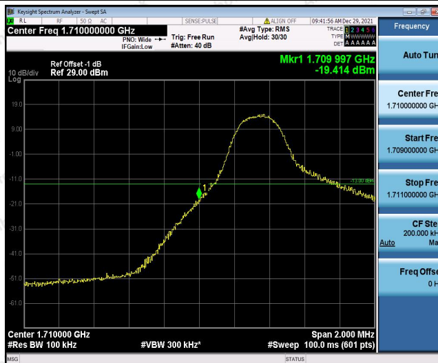
Band4-5MHz-16QAM-19975-1RB#24
