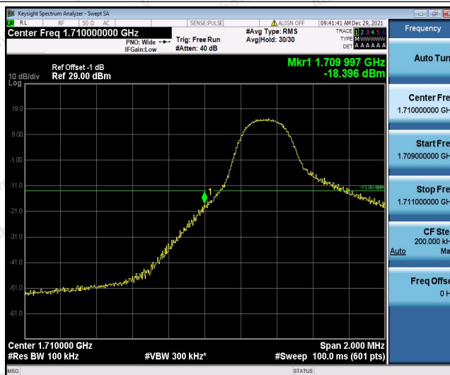
Band4-5MHz-QPSK-19975-1RB#24
