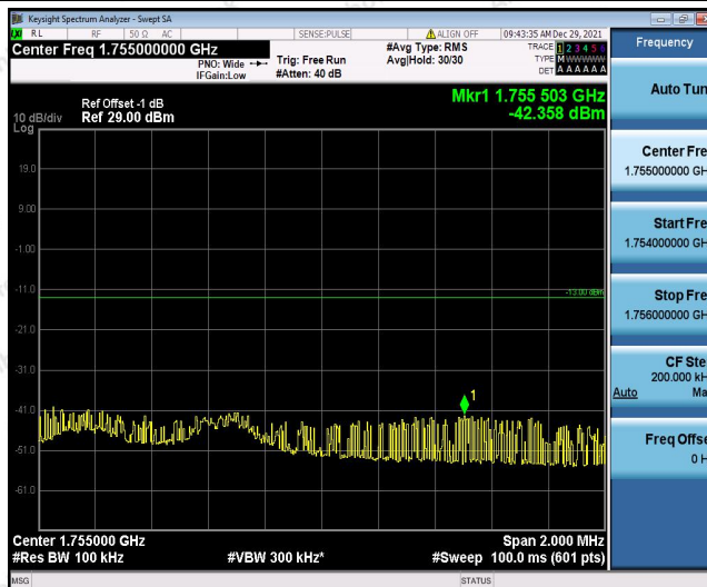
Band4-5MHz-16QAM-20375-1RB#24
