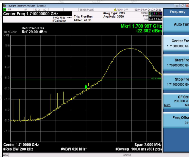
Band4-10MHz-QPSK-20000-1RB#49
