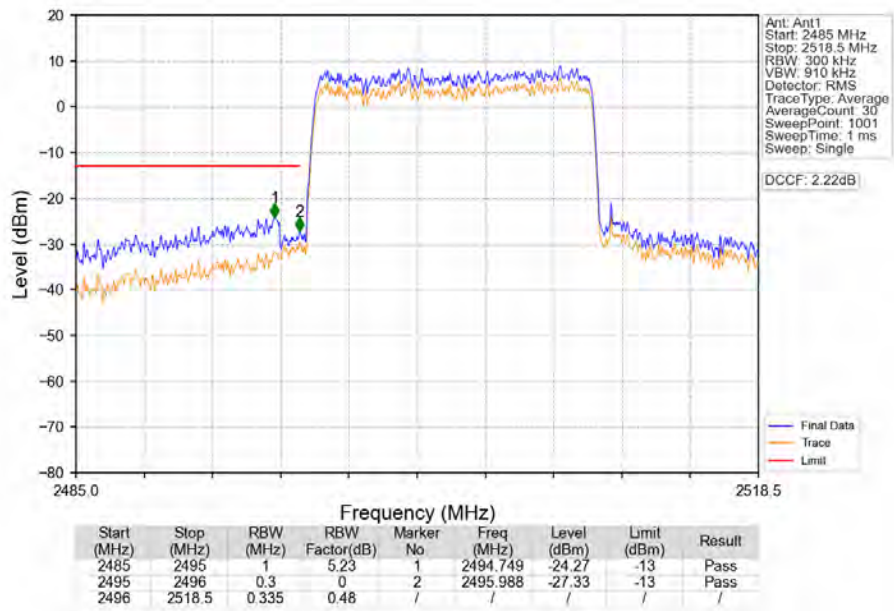
Band41_15MHz_16QAM_LCH_2503.5MHz_RB_75_0_NTNV
