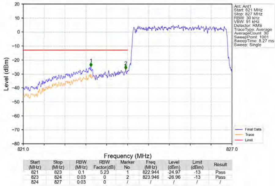
Band26b_3MHz_16QAM_LCH_825.5MHz_RB_15_0_NTNV
