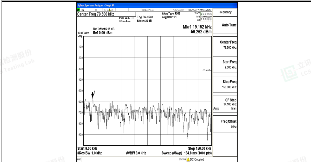
Band12_10MHz_16QAM_23060_1RB#0_0.009~0.15_0.009~0.15
