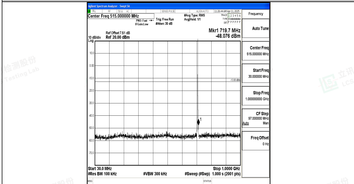
Band12_1.4MHz_16QAM_23173_1RB#0_30~1000_30~1000
