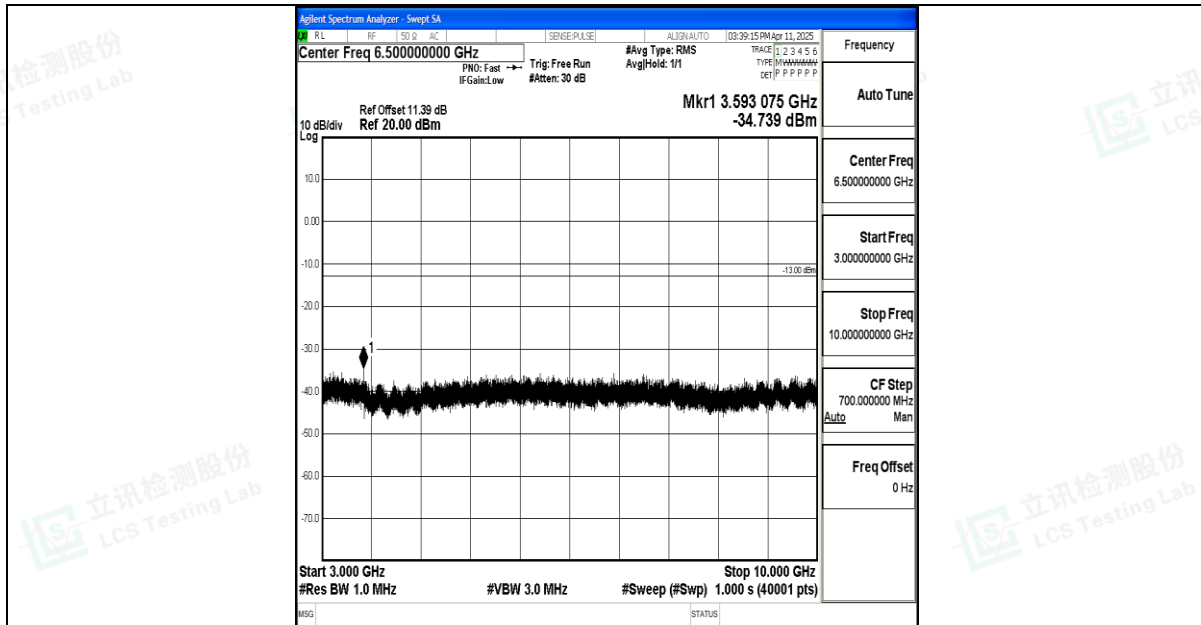
Band12_10MHz_QPSK_23060_1RB#0_3000~10000_3000~10000
