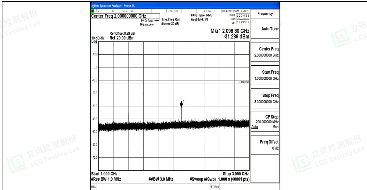
Band12_10MHz_16QAM_23060_1RB#0_1000~3000_1000~3000
