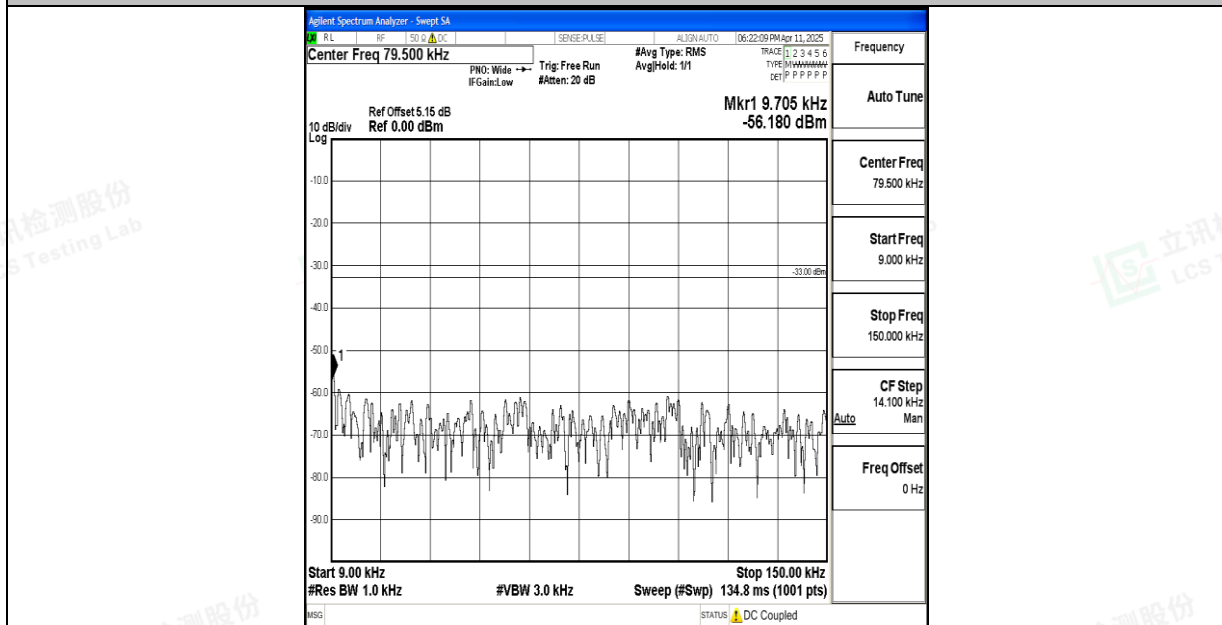
Band26_10MHz_QPSK_26740_1RB#0_0.009~0.15_0.009~0.15
