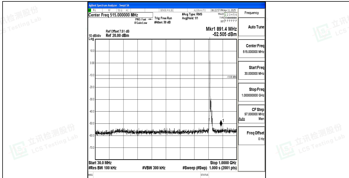
Band26_10MHz_16QAM_26740_1RB#0_30~1000_30~1000
