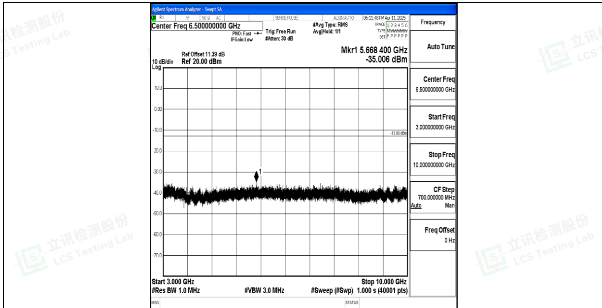
Band26_5MHz_16QAM_26765_1RB#0_3000~10000_3000~10000
