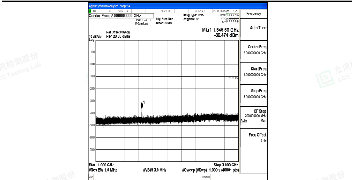
Band26_1.4MHz_16QAM_26783_1RB#0_1000~3000_1000~3000
