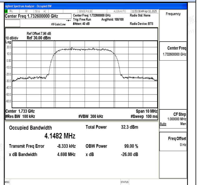
Channel 1413 / 1732.6 MHz
