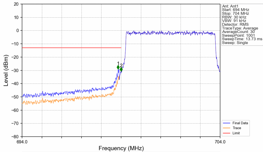
Band12_5MHz_16QAM_LCH_701.5MHz_RB_25_0_NTNV
