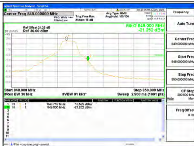
B26 Part22 / 1.4MHz / High CH / QPSK / 1 RB
