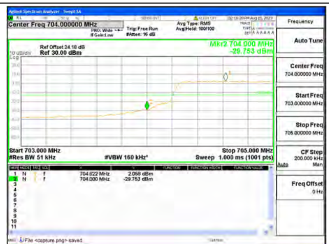
B17 / 5MHz / Low CH / QPSK / FULL RB
