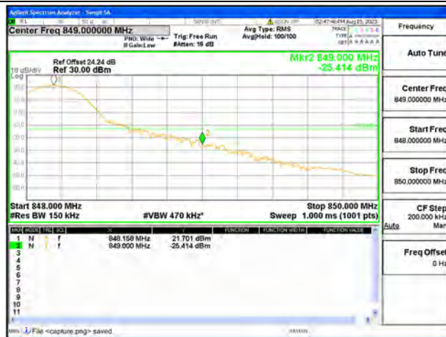
B26 Part22 / 15MHz / High CH / QPSK / 1 RB
