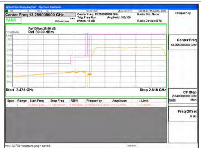
B41 / 20MHz / Low CH / QPSK / FULL RB
