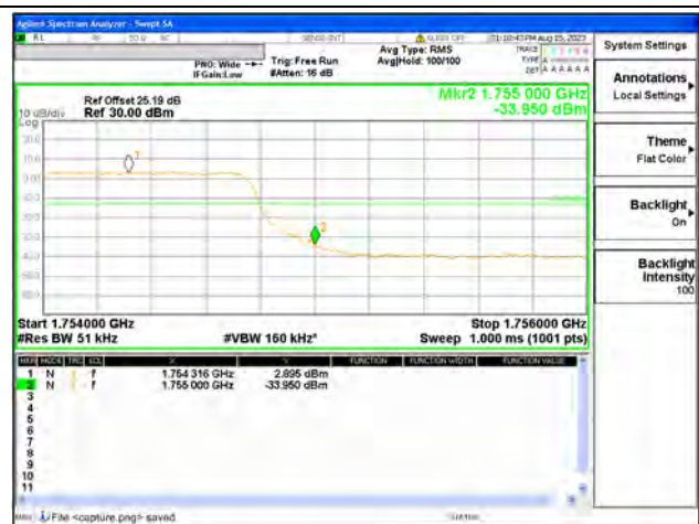
B4 / 5MHz / High CH / QPSK / FULL RB
