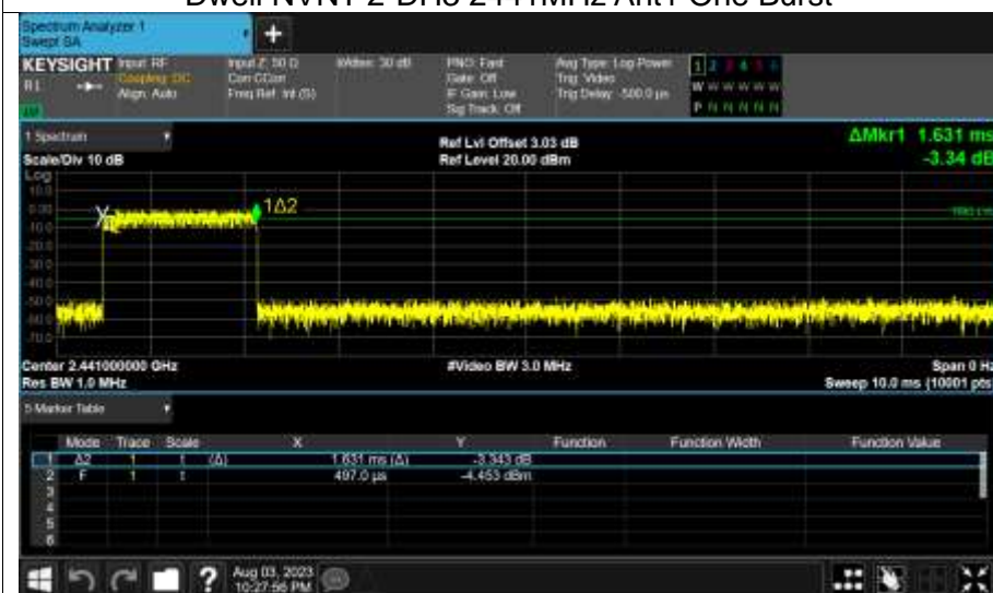
Dwell NVNT 2-DH3 2441MHz Ant1 One Burst
