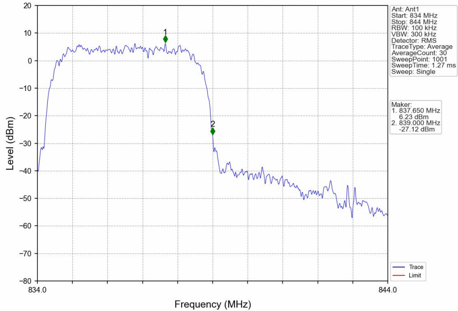
Band5_HSDPA_MCH_836.6MHz_Subtest 1_NTNV
