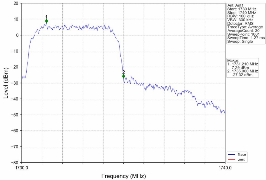
Band4_HSDPA_MCH_1732.6MHz_Subtest 1_NTNV
