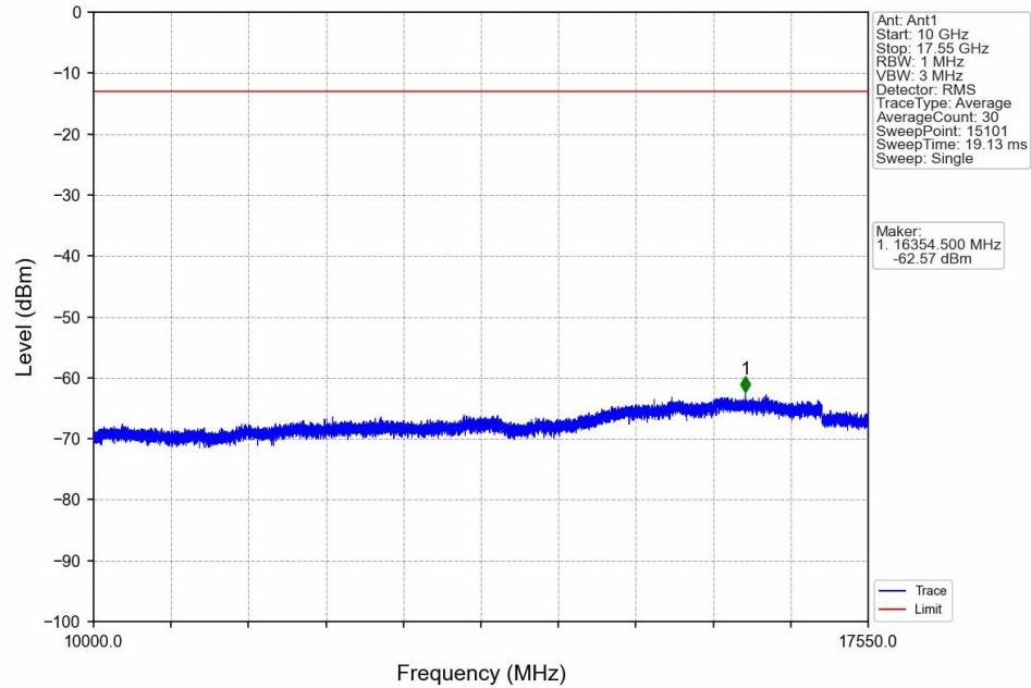
Band4_HSUPA_MCH_1732.6MHz_Subtest 1_NTNV
