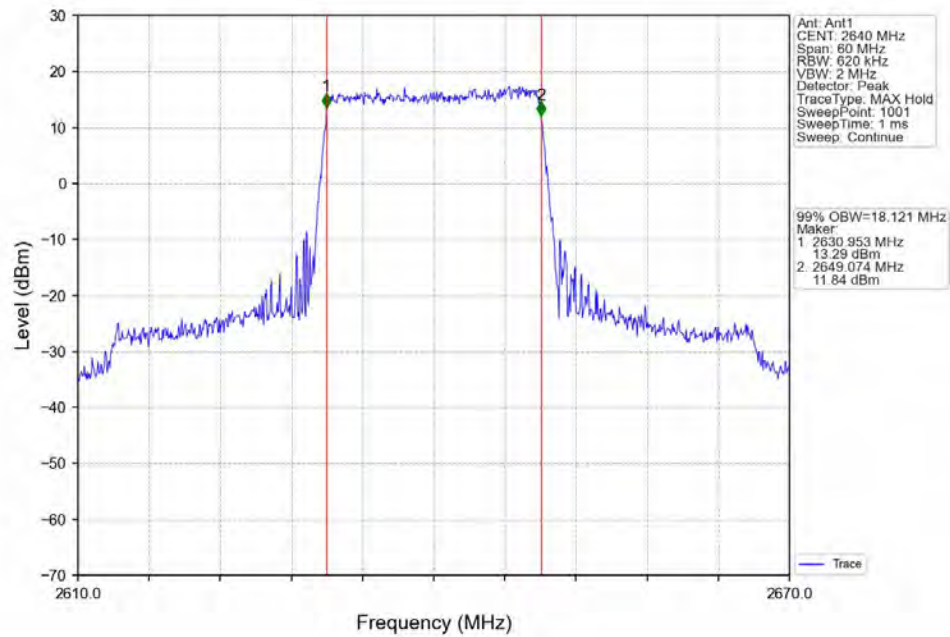
Band41_20MHz_16QAM_HCH_2640MHz_RB_100_0_NTNV
