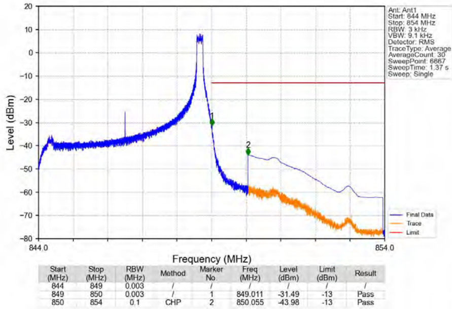
Band26b_5MHz_16QAM_HCH_846.5MHz_RB_1_24_NTNV
