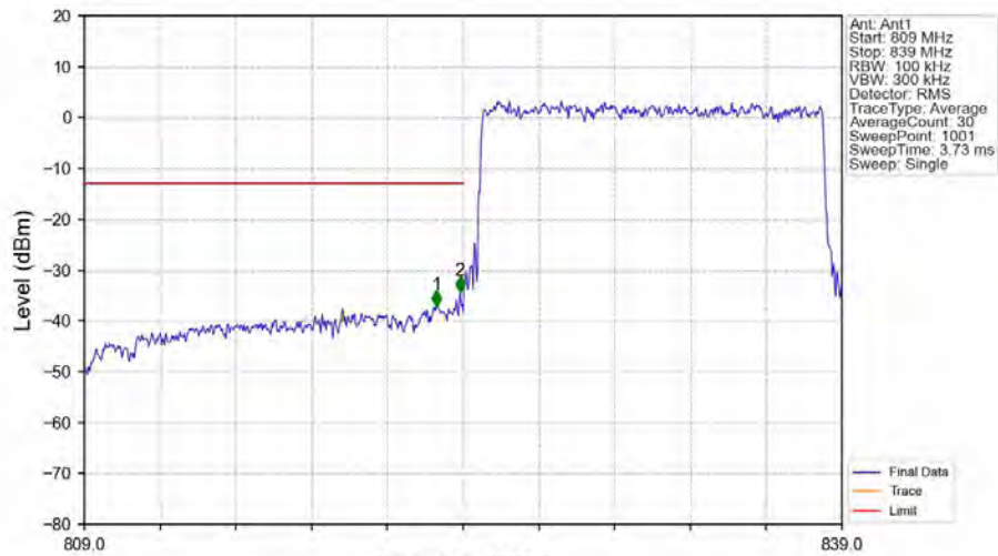
Band26b_15MHz_16QAM_LCH_831.5MHz_RB_75_0_NTNV
