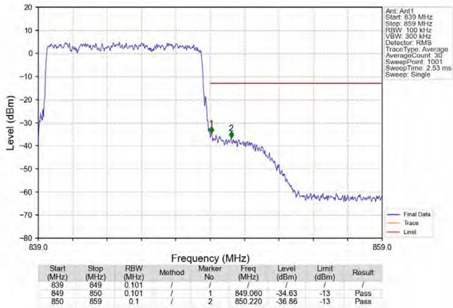
Band26b_10MHz_16QAM_HCH_844MHz_RB_50_0_NTNV
