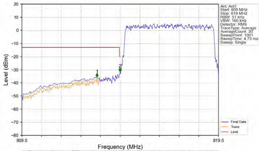
Band26a_5MHz_16QAM_LCH_816.5MHz_RB_25_0_NTNV
