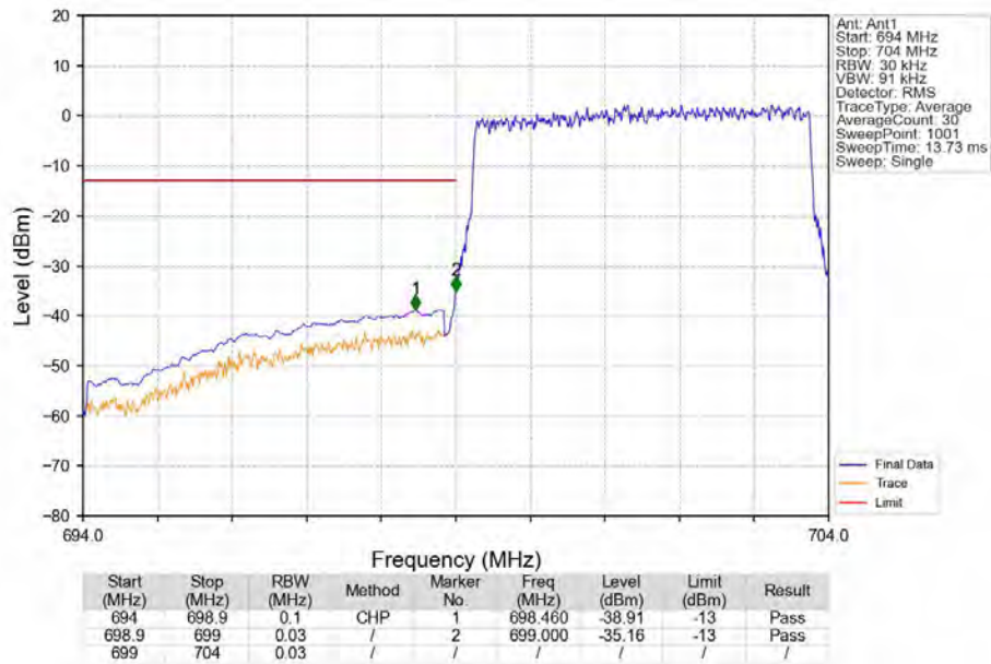
Band12_5MHz_16QAM_LCH_701.5MHz_RB_25_0_NTV
