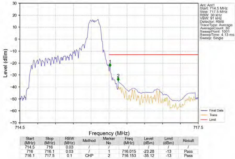
Band12_1.4MHz_16QAM_HCH_715.3MHz_RB_1_5_NTNV
