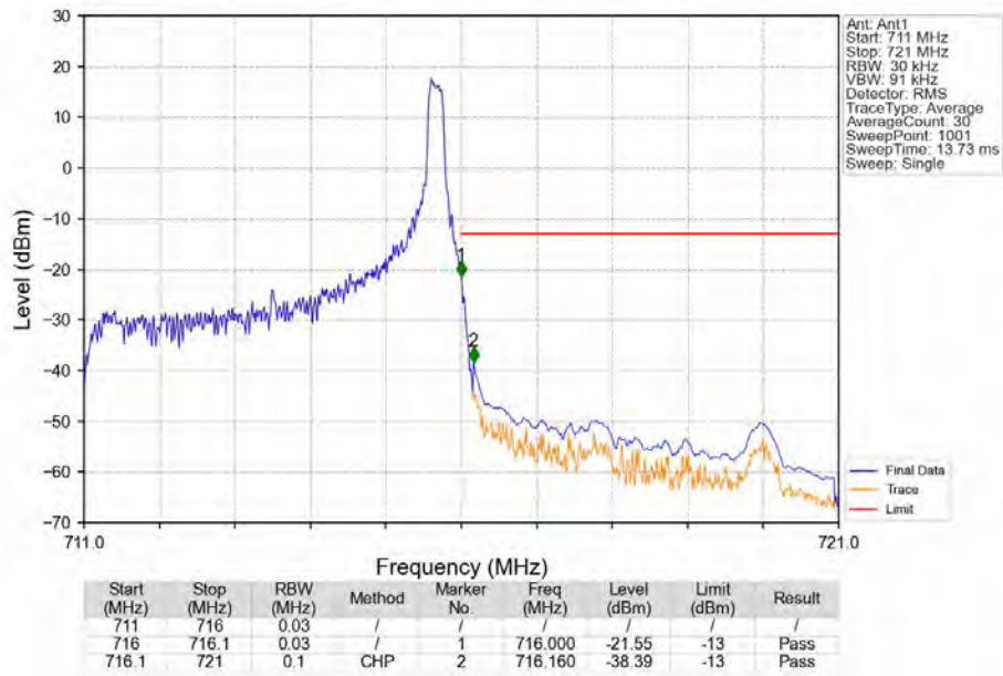
Band12_5MHz_QPSK_HCH_713.5MHz_RB_1_24_NTNV
