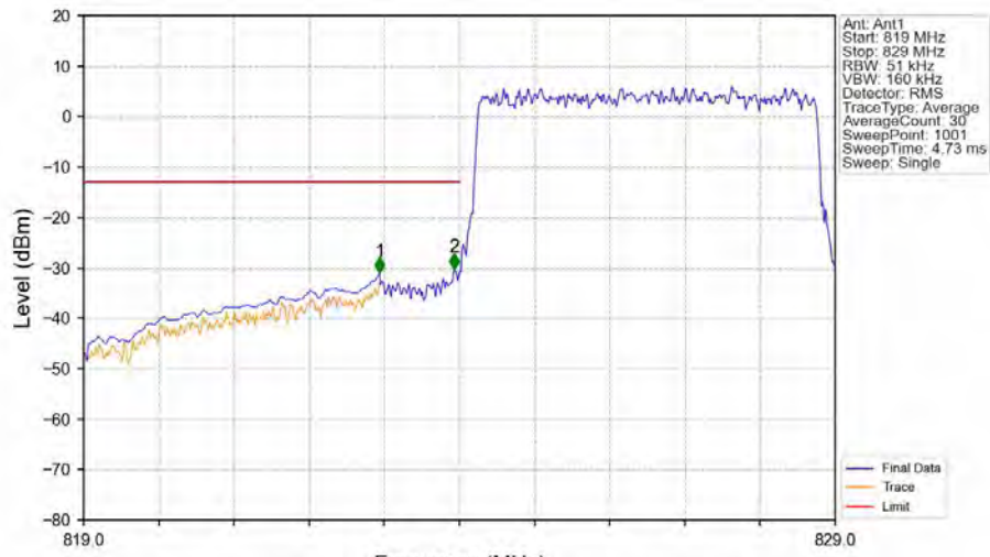
Band5_5MHz_16QAM_LCH_826.5MHz_RB_25_0_NTNV
