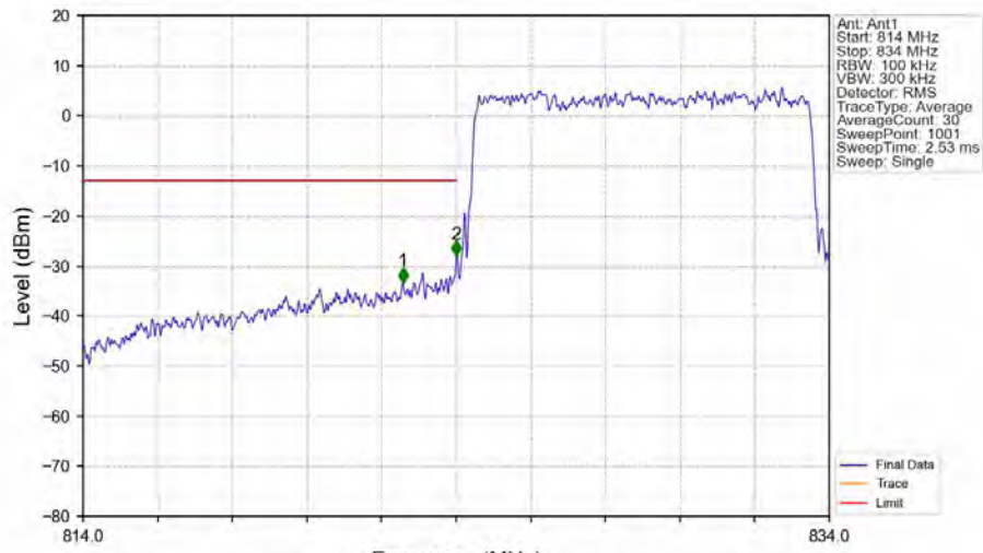
Band5_10MHz_16QAM_LCH_829MHz_RB_50_0_NTNV
