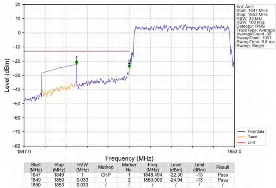
Band2_3MHz_QPSK_LCH_1851.5MHz_RB_15_0_NTNV
