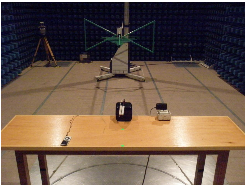
Rear view (Charging and Aux-in)
