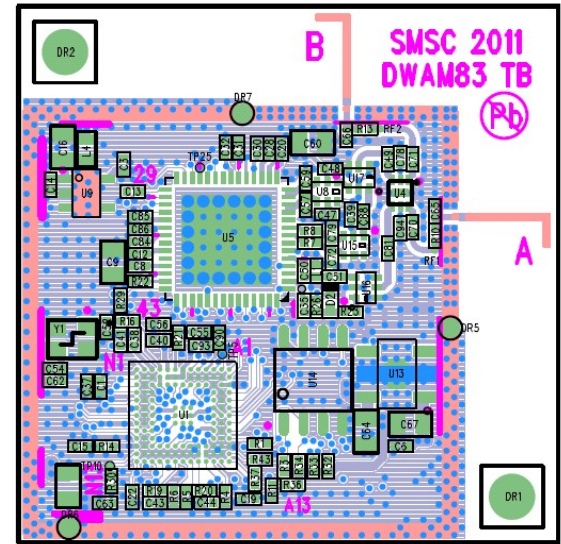
TOP-SIDE
