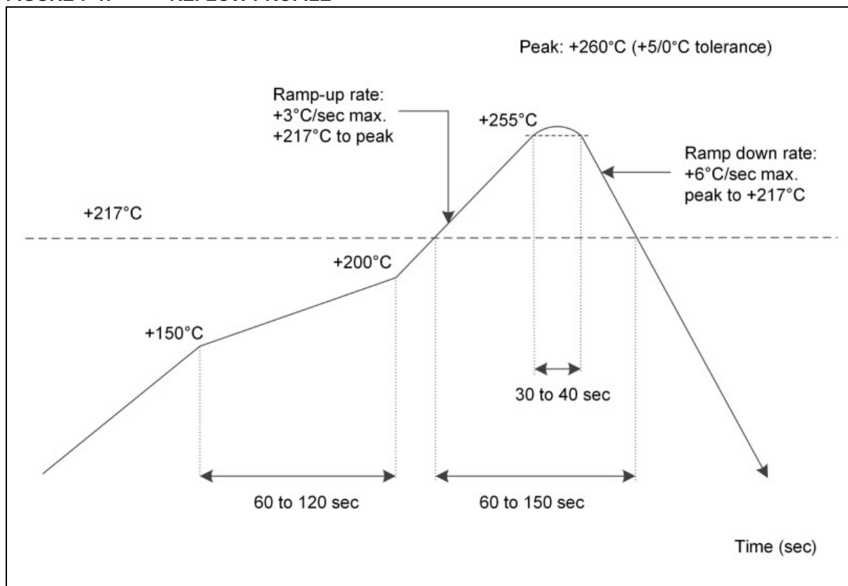
FIGURE 7-1: REFLOW PROFILE
