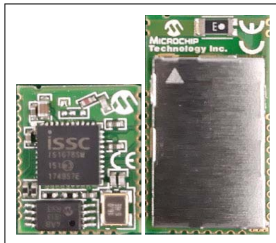
FIGURE 1: BM78 MODULE
