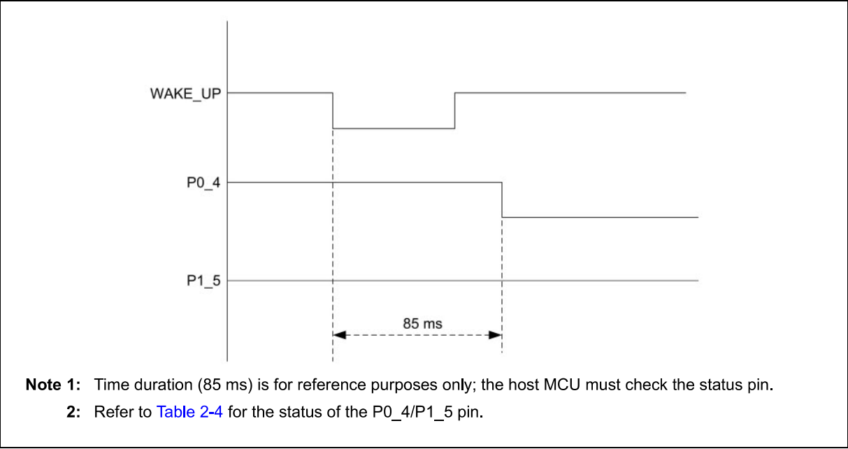
FIGURE 2-5: WAKE-UP TIME
