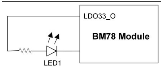
FIGURE 2-7: LED DRIVER
