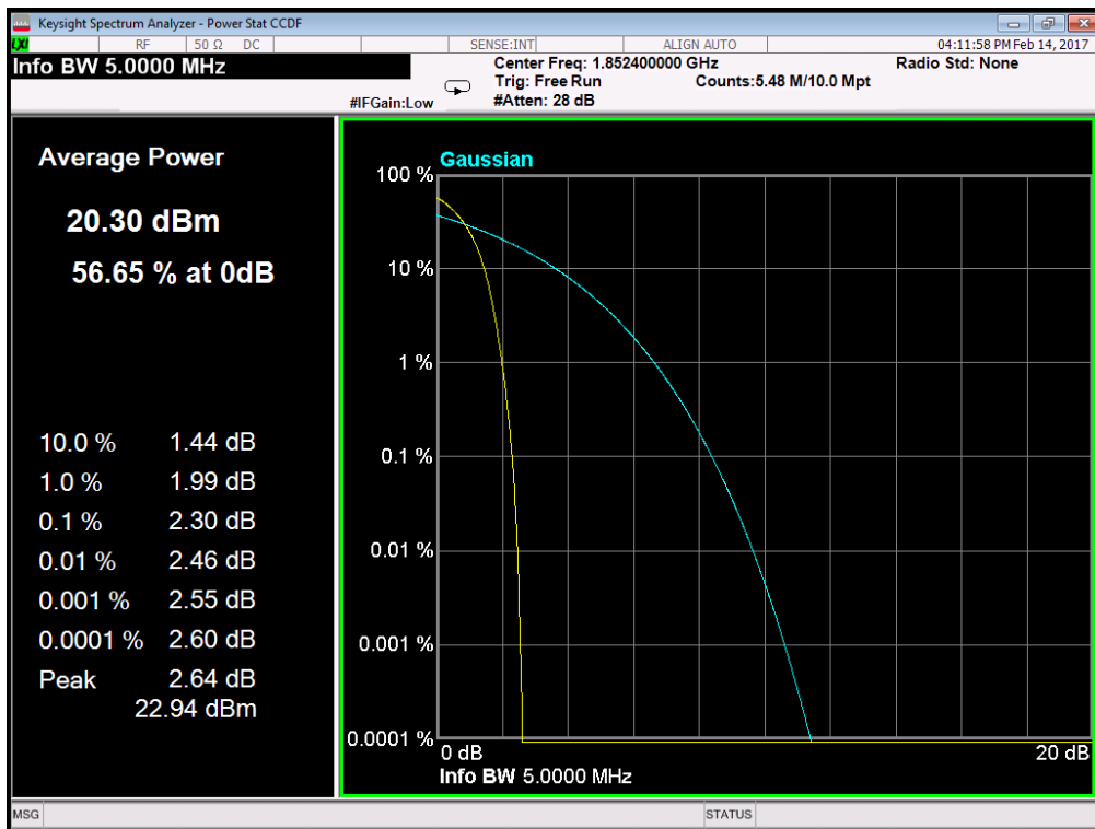
(Plot A1: WCDMA 1900MHz Channel = 9262)
