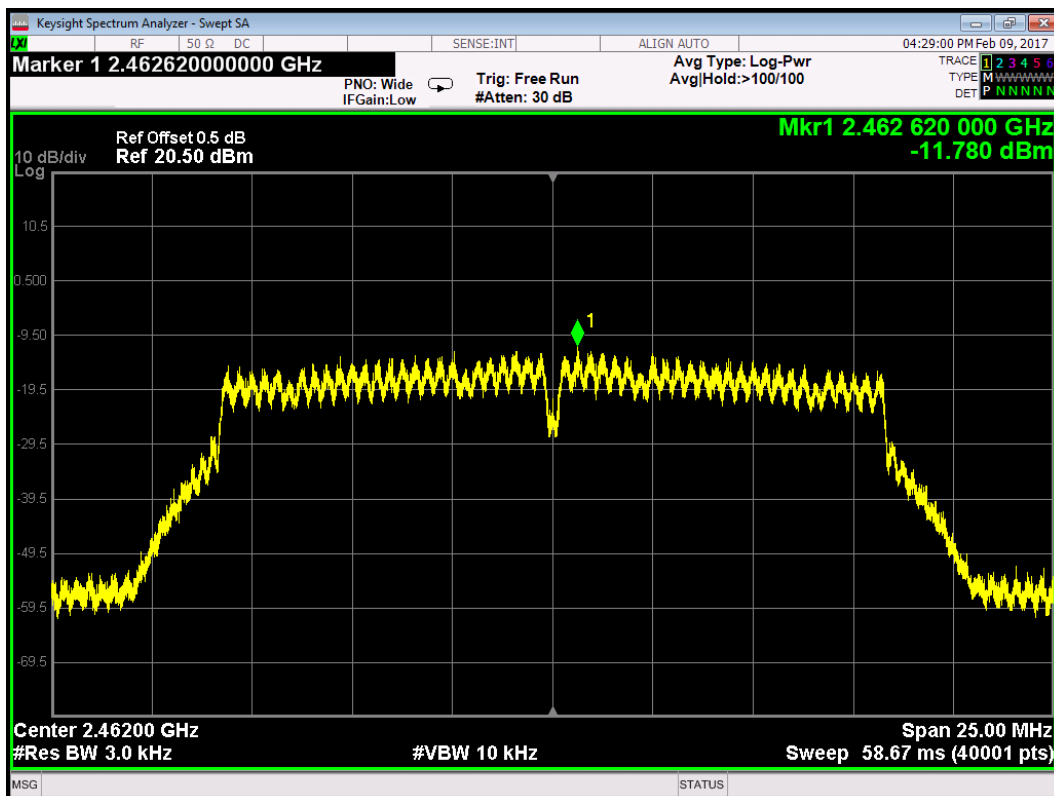
802.11g - Channel 11
