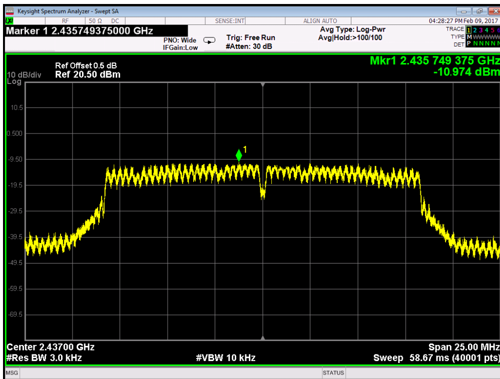
802.11g - Channel 6
