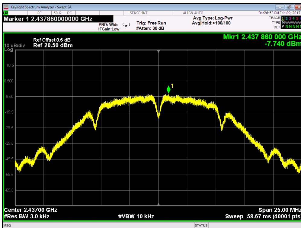
802.11b - Channel 6
