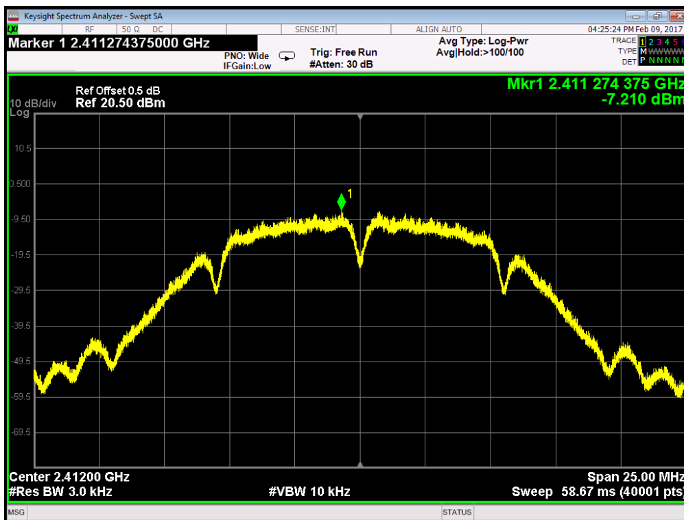
802.11b - Channel 1
