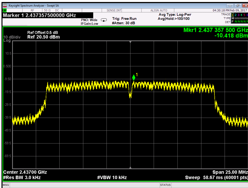
802.11n20 - Channel 6
