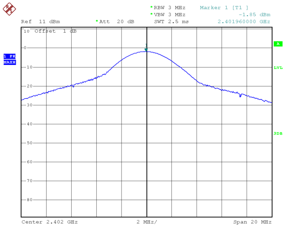
Plot C1:8-DPSK
