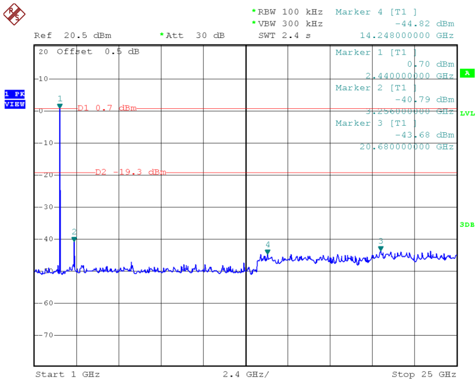
(Plot B.2: Channel = 19, 1GHz to 25GHz)
