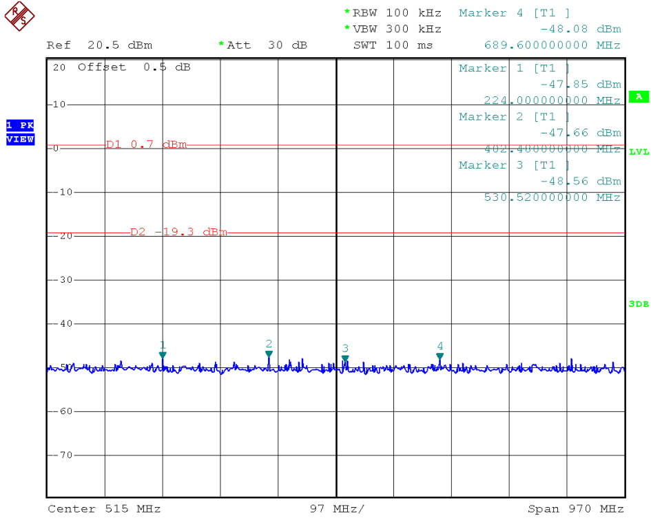
(Plot B.1: Channel = 19, 30MHz to 1GHz)
