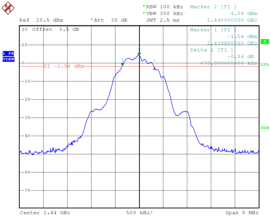
(Plot B1: Channel 19: 2440 MHz)
