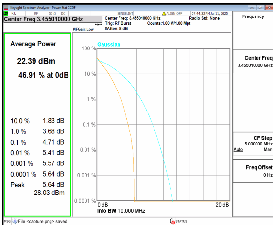
n77(3450-3550MHz) 10M DFT-s-OFDM Outer_Full Low
