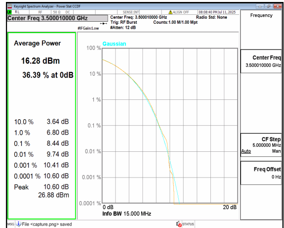
n77(3450-3550MHz) 15M CP-OFDM 256QAM Outer_Full Mid
