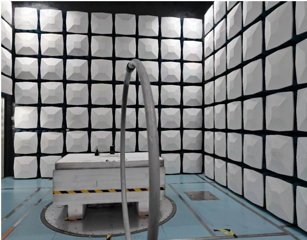
Radiated Emission 9k-30MHz Perpendicular View
