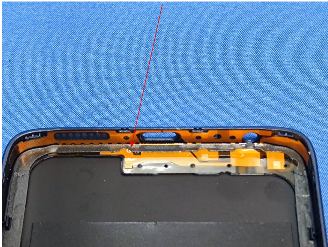
WWAN Div Antenna(Above 1G Frequency Band)
