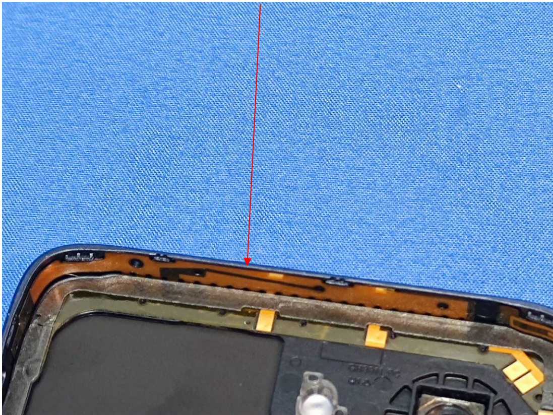
WWAN Main Antenna(Below 1G Frequency Band)
