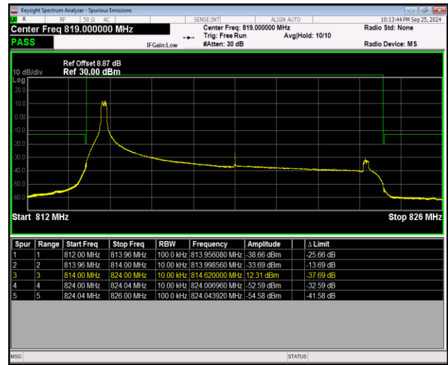
Band26-10MHz-16QAM-26740-50RB#0
