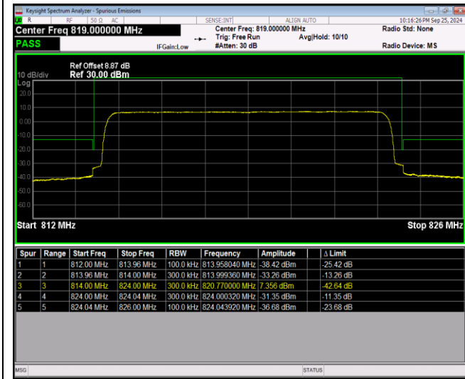
Band26-10MHz-16QAM-26740-1RB#49
