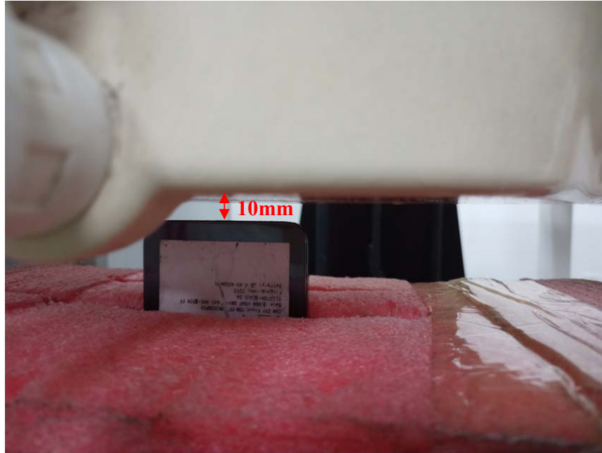
Body Bottom Setup Photo (10mm)
