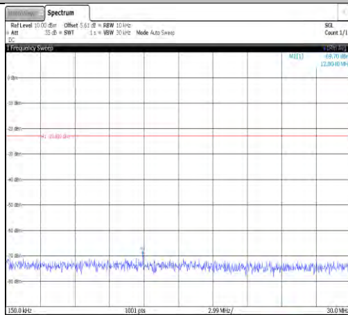
Band5-4182-3-0.15~30MHz-PASS
