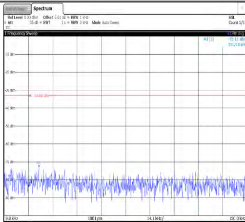
Band5-4182-3-0.009~0.15MHz-PASS
