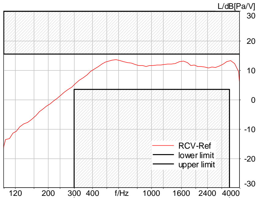
Figure C.4-2 – WLAN 2.4GHz 8N FF Narrowband Frequency Response
