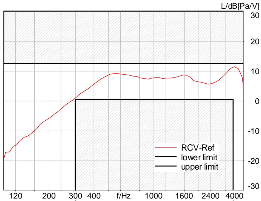
Figure C.4-1 – WLAN 2.4GHz 2N FF Narrowband Frequency Response
