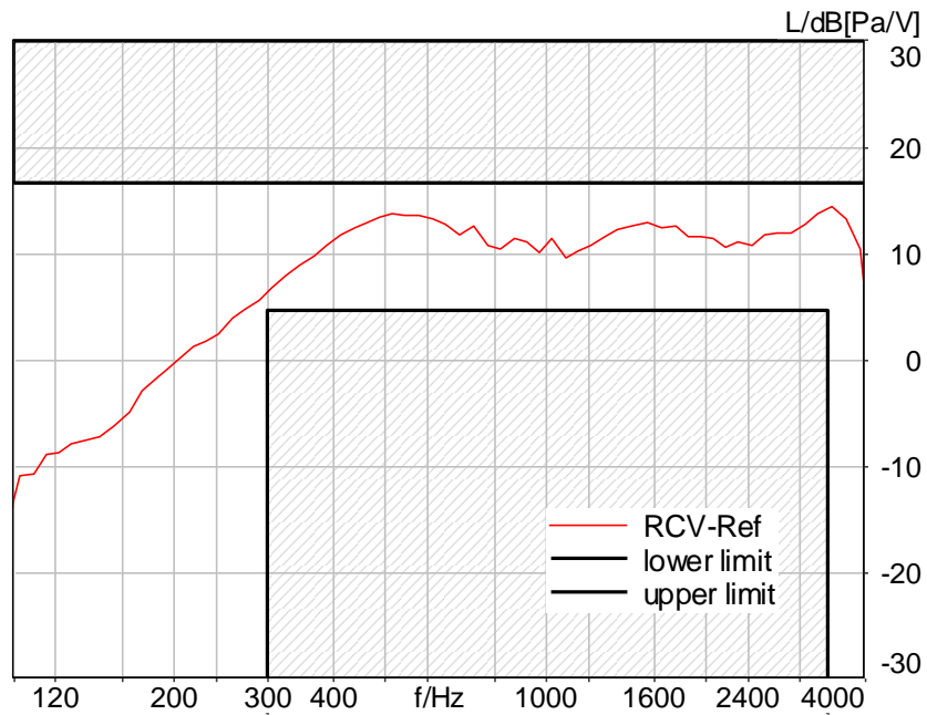
Figure C.3-2 – LTE Band 2 8N FF Narrowband Frequency Response
