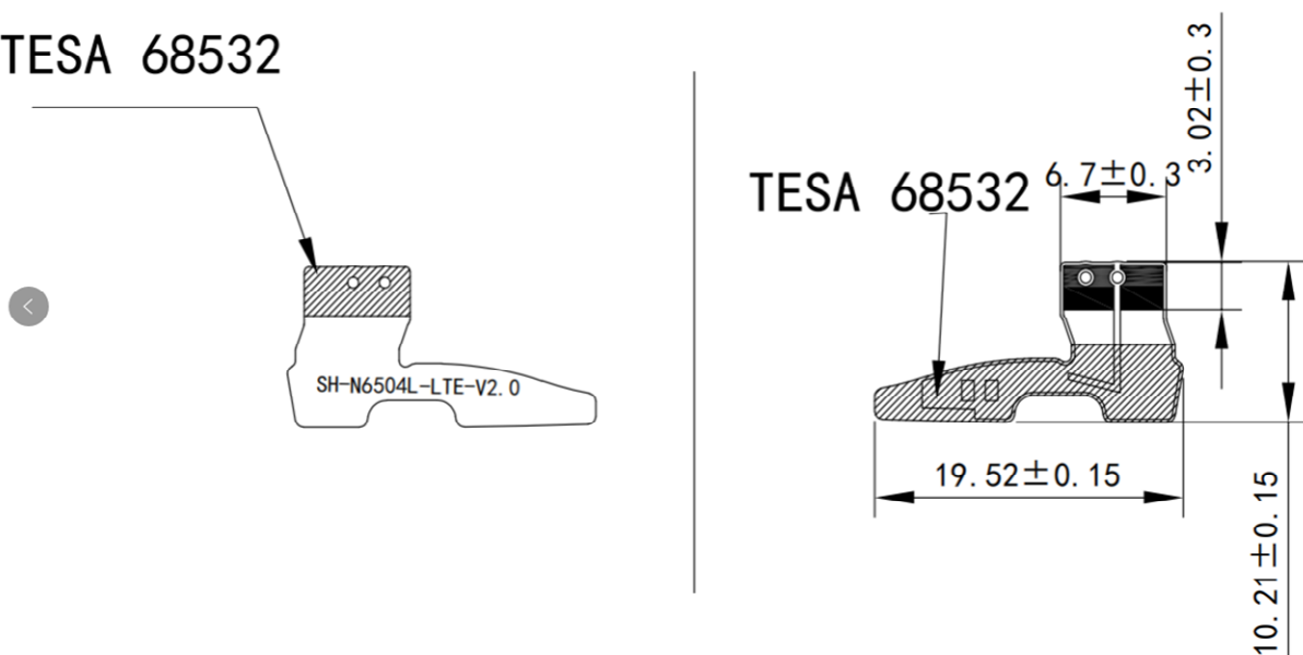
Diversity antenna
